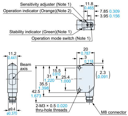
CX-41□-Z Sensor
