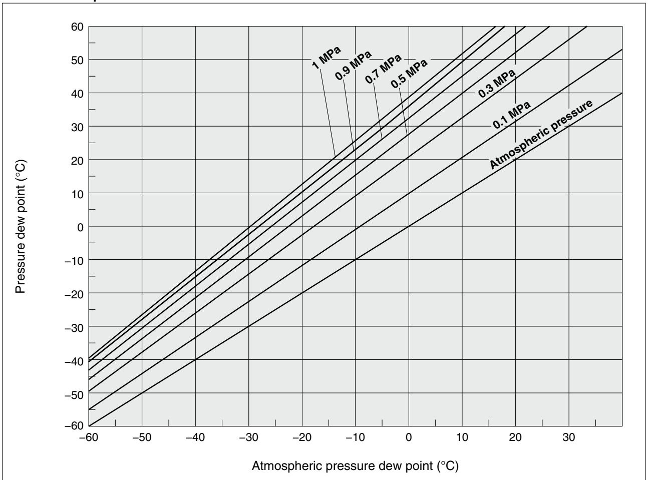
Dew Point Temperature Conversion Chart
